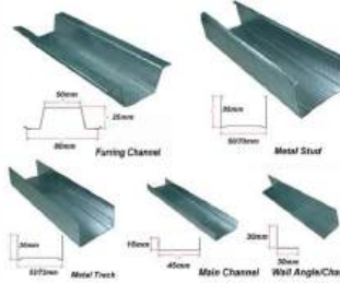
GYPSUM BOARD FITTINGS
